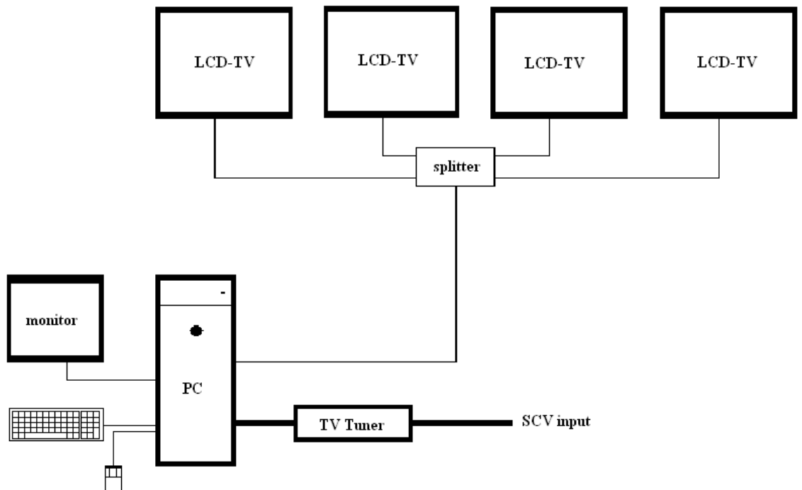
Schematic layout
